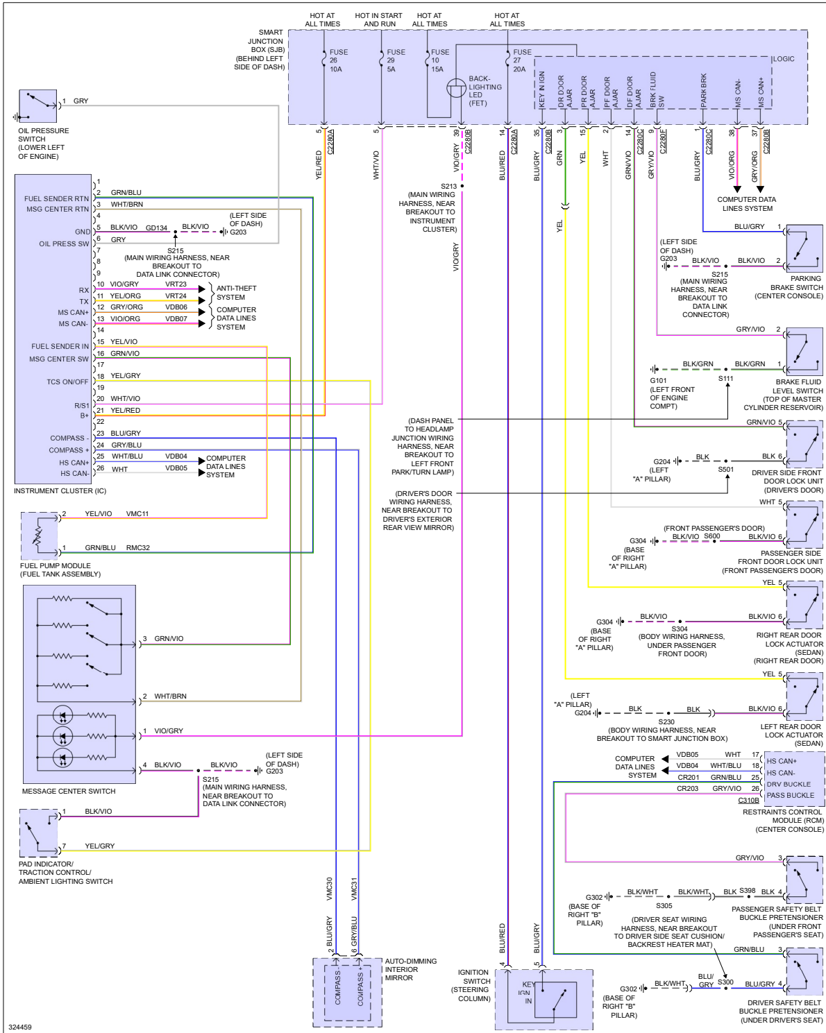
Fig 1: Instrument Cluster Circuit
